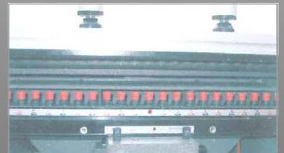
◆ Boring unit pneumatically tiltable vertical to horizontal
